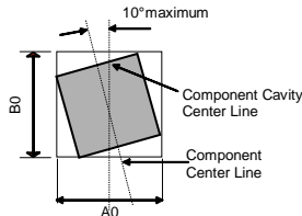
Sketch B (Top View) Component Rotation
